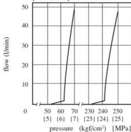
MB*-03-~-10T pressure drop characteristic
