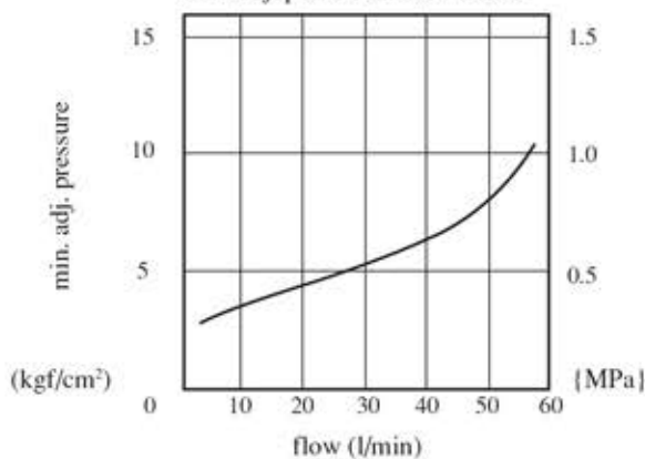
MB*-03-B-10T min. adj. pressure characteristic
